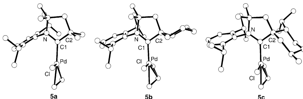
Figure 3. Molecular view of the crystal structures of 5a–c . Selected lengths [Å] and angles [°]: 5a : N–C1 1.3133(11), C1–C2 1.5298(12), C1–Pd 2.0246(9); N–C1–C2 108.51(8). 5b : N–C1 1.310(4), C1–C2 1.526(4), C1–Pd 2.020(3); N–C1–C2 108.7(2). 5c : N–C1 1.315(5), C1–C2 1.543(5), C1–Pd 2.045(4); N–C1–C2 108.8(3).
