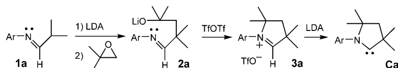
Scheme 2. Synthesis of CAAC Ca . Ar = 2,6-diisopropylphenyl.
