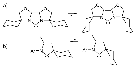
Scheme 3. Flexible steric bulk for a) NHCs ( B ) and b) CAACs ( Cb ). Ar = 2,6-diisopropylphenyl.
