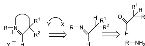
Scheme 1. Retrosynthetic analysis for the preparation of CAACs.
