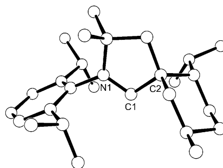
Figure 2. Molecular view of the crystal structure of Cc . Selected bond lengths [Å] and angles [°]: N1–C1 1.315(3), C1–C2 1.516(3); N1–C1–C2 106.54(18).
