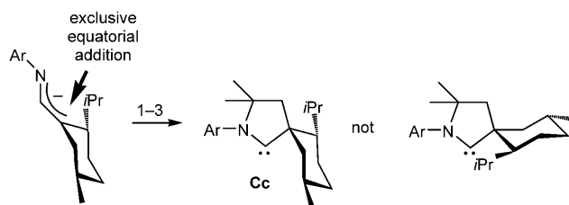
Scheme 4. Stereoselective synthesis of CAAC Cc . 1) Dimethyloxirane; 2) TfOTf; 3) LDA; Ar = 2,6-diisopropylphenyl.
