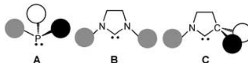
Figure 1. Schematic view of ligands A–C showing their different steric demands.
